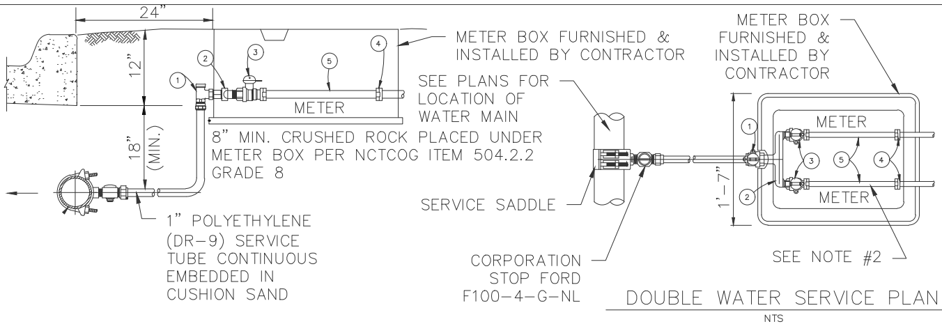
DOUBLE WATER SERVICE SECTION
