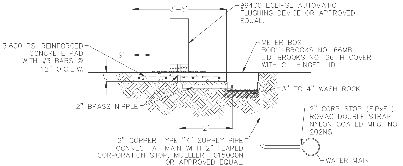
ELEVATION VIEW
