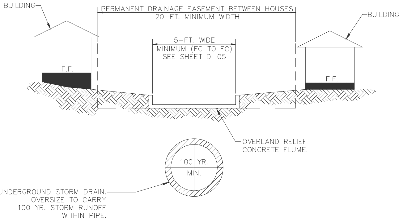
STORM DRAIN BETWEEN HOUSES IN SUMP
