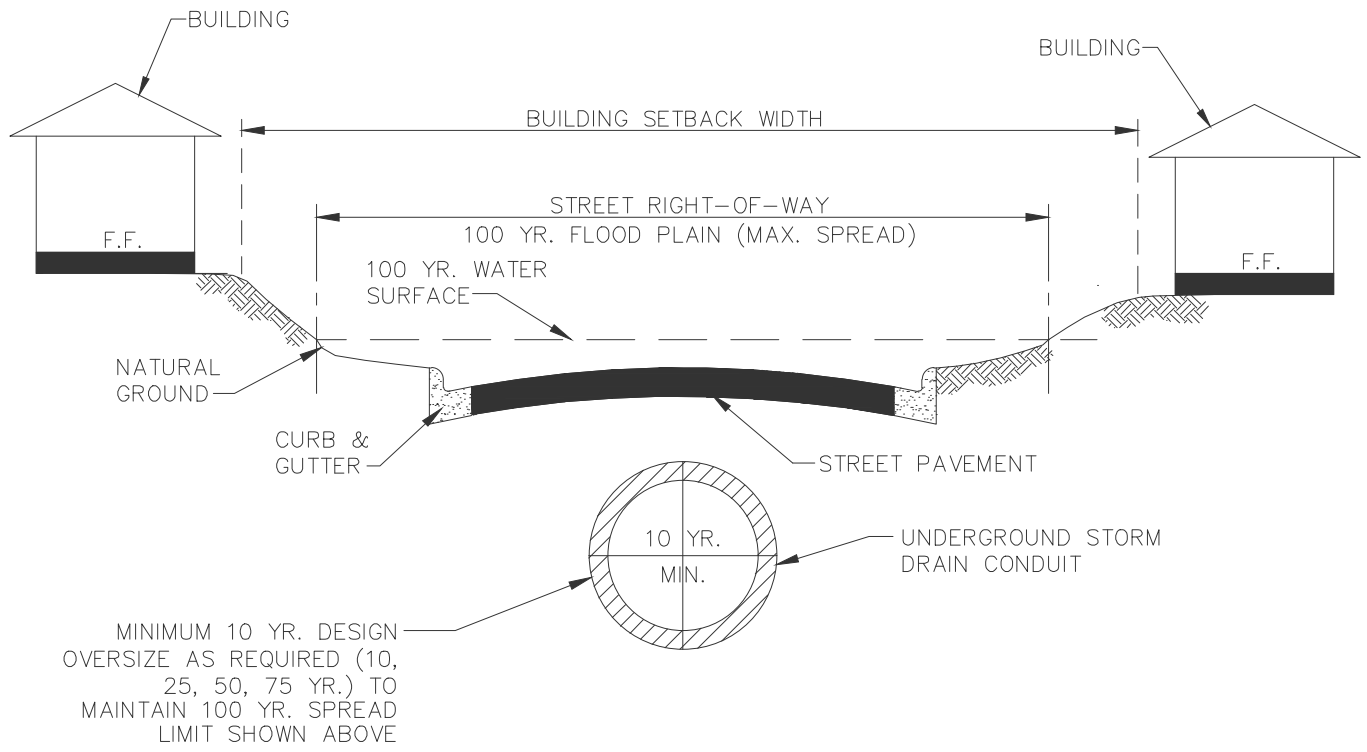
STORM DRAIN IN STREET
