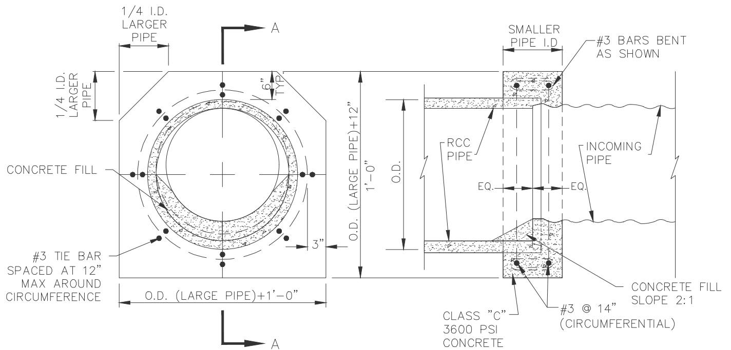
COUPLING OF RCCP TO PIPE OF ANOTHER MATERIAL
