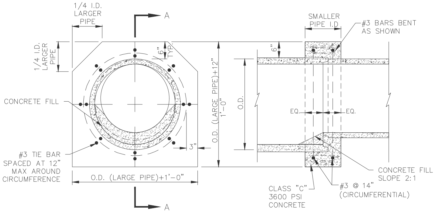
COUPLING OF R.C.C. PIPES OF DIFFERENT DIAMETERS
