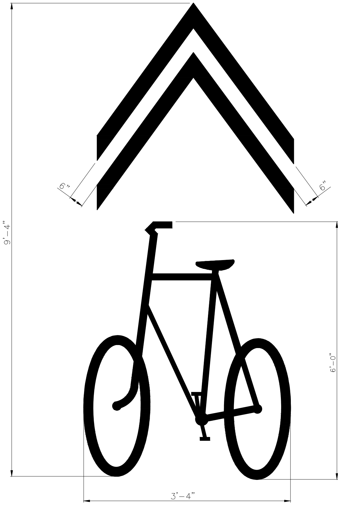
BICYCLE SHARED LANE MARKING NTS
